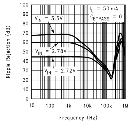
Figure 22. Ripple Rejection
