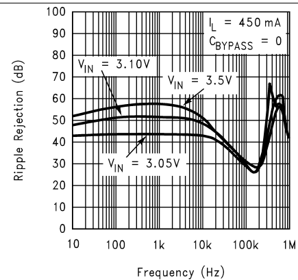
Figure 24. Ripple Rejection
