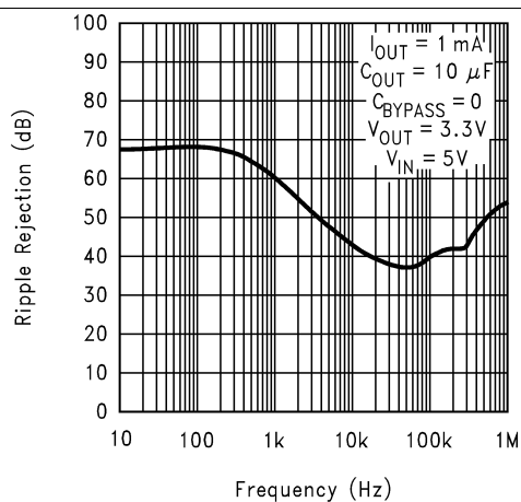
Figure 6. Ripple Rejection
