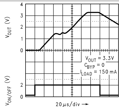
Figure 30. Turnon Time
