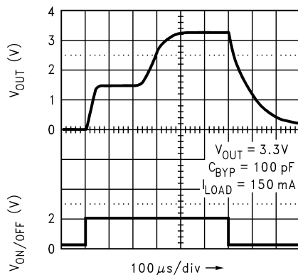
Figure 5-51. Turn-on Time for Legacy Chip
