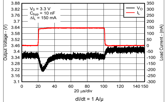
Figure 5-38. Load Transient for New Chip
