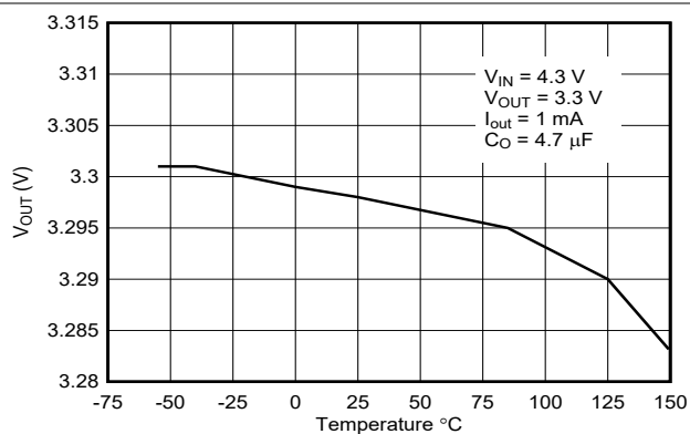
Figure 5-2. V_{OUT} vs Temperature for New Chip
