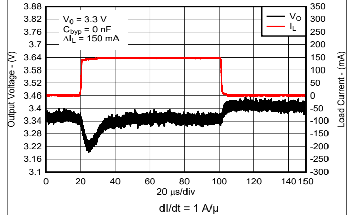
Figure 5-40. Load Transient Response for New Chip
