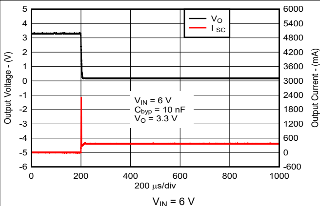
Figure 5-4. Short-Circuit Current vs Time for New Chip
