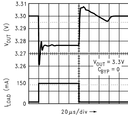
Figure 5-37. Load Transient Response for Legacy Chip
