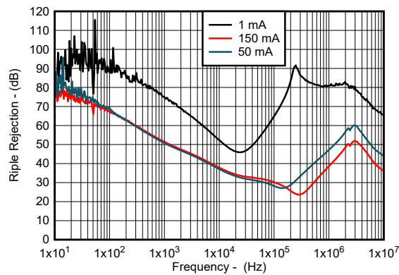
V_{IN} = 3.7 V , V_{OUT} = 3.3 V , C_{OUT} = 10 \mu F , C_{BYP} = 0 nF Figure 5-17. Ripple Rejection vs Frequency for New Chip
