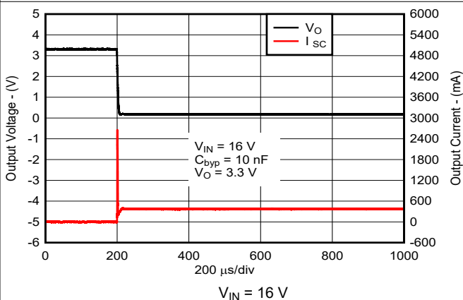
Figure 5-6. Short-Circuit Current vs Time for New Chip
