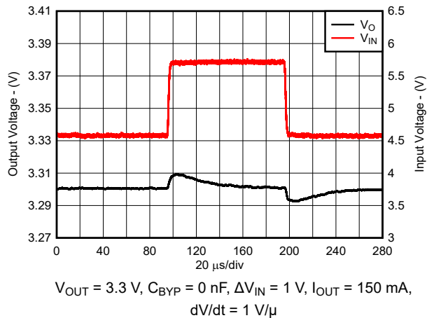
Figure 5-46. Line Transient Response for New Chip
