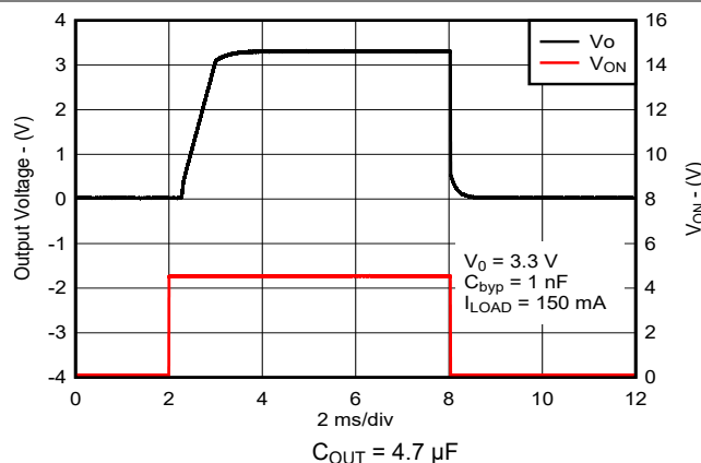
Figure 5-56. Turn-on Time for New Chip
