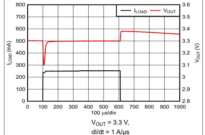
Figure 5-42. Load Transient Response for New Chip
