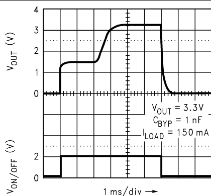
Figure 5-55. Turn-on Time for Legacy Chip
