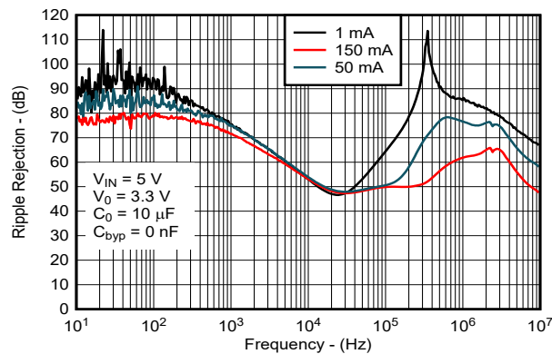
V_{IN} = 5 V , V_{OUT} = 3.3 V , C_{OUT} = 10 \mu F , C_{BYP} = 0 nF Figure 5-13. Ripple Rejection vs Frequency for New Chip
