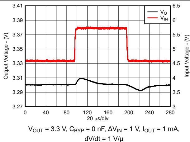
Figure 5-44. Line Transient Response for New Chip
