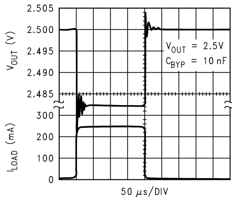
Figure 5-39. Load Transient Response for Legacy Chip
