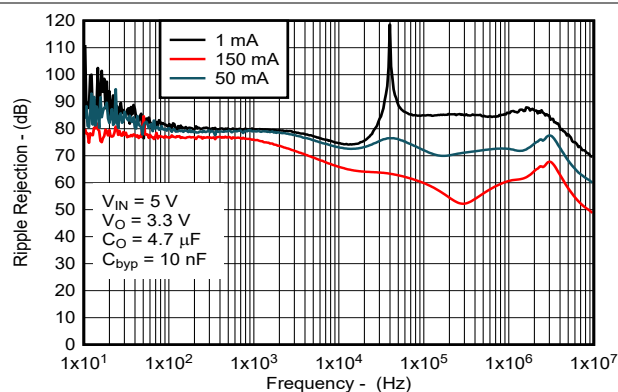
Figure 5-20. Ripple Rejection vs Frequency for New Chip
