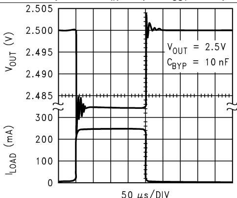
Figure 25. Load Transient Response
