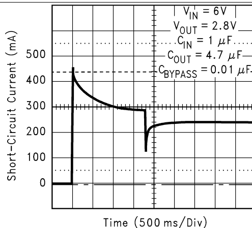
Figure 2. Short-Circuit Current
