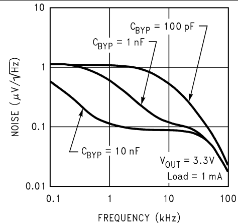
Figure 16. Output Noise Density
