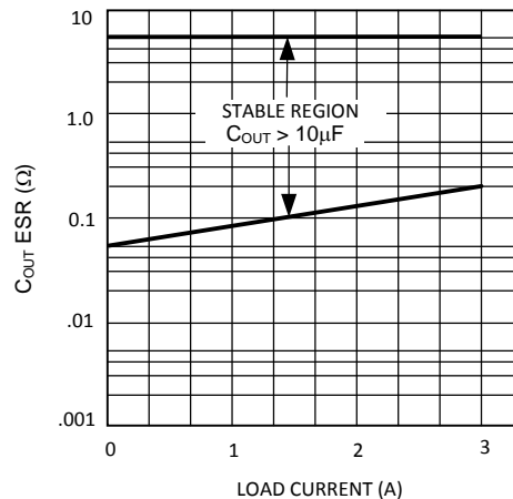
Figure 28. ESR Curve for C_{OUT} (with 10\mu\text{F} Tantalum Input Capacitor)
