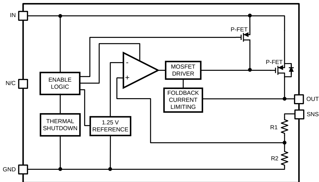
Figure 27. LP38690 Functional Diagram (WSN)
