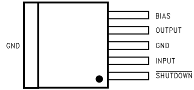
Figure 2. DDPACK/TO-263, Top View
