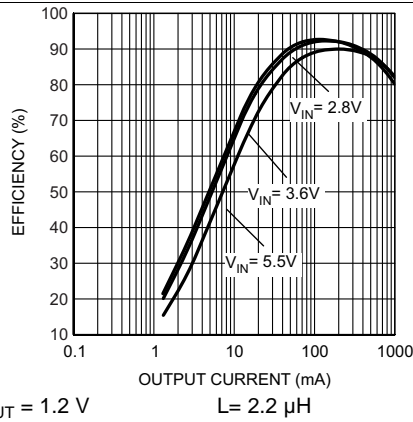
Figure 14. Efficiency vs Output Current (Forced PWM Mode)
