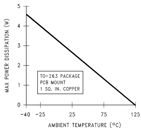
Figure 24. Maximum power dissipation vs ambient temperature for DDPAK/TO-263 package
