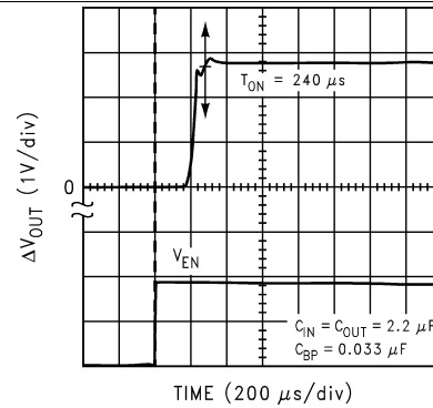
Figure 14. Enable Response ( t_{ON} )
