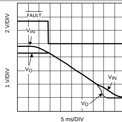
Figure 12. Power-Down Response
