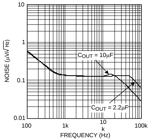
Figure 7. Output Noise Spectral Density
