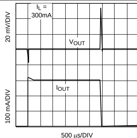
Figure 20. Load Transient
