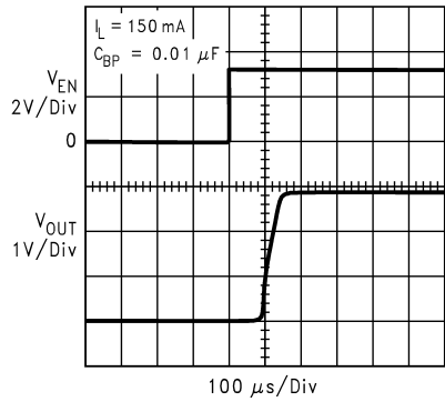
Enable Response ( V_{IN} = V_{OUT} + 0.2V )
