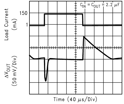
Load Transient Response ( V_{IN} = 4.2V )
