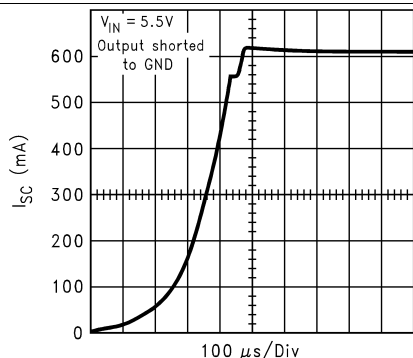
Figure 15. Short Circuit Current (DSBGA)
