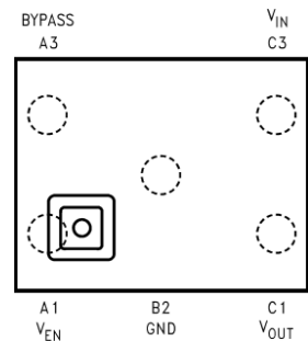
Figure 4. Top View 5-Bump DSBGA Package Package Number TLA05
