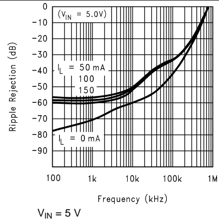
Figure 18. Ripple Rejection
