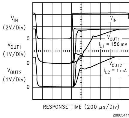
Enable Response ( V_{IN} = V_{OUT} + 0.2\text{V} )
