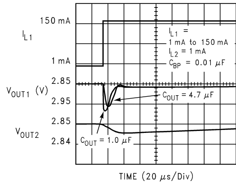
Load Transient & Cross Talk ( V_{IN} = V_{OUT} + 0.2\text{V} )
