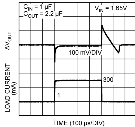
Figure 15. Load Transient
