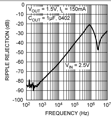
Figure 2. Power Supply Rejection Ratio
