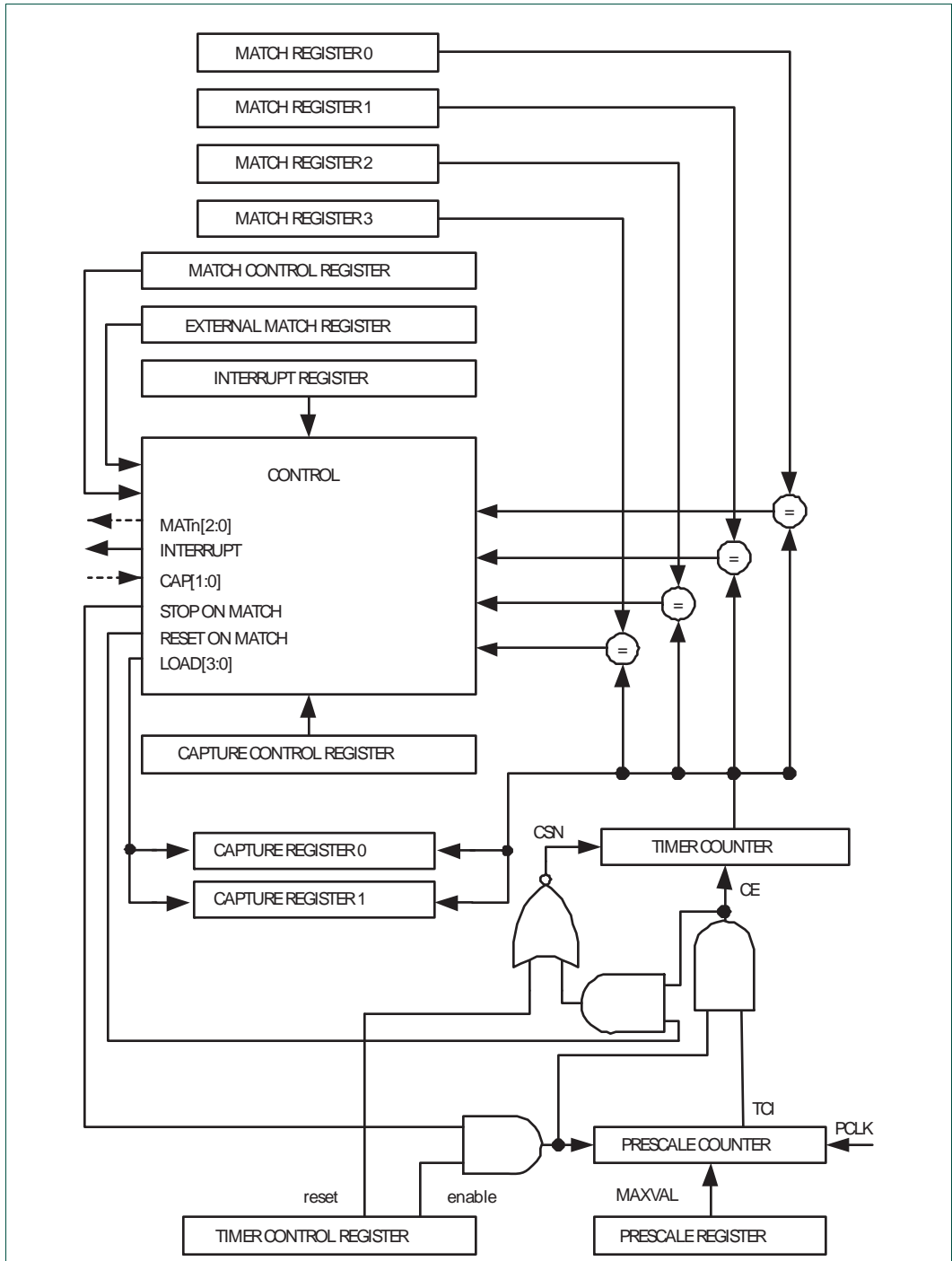
Fig 76. 16-bit counter/timer block diagram
