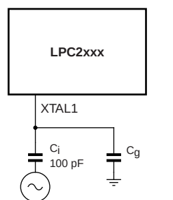
Fig 27. Slave mode operation of the on-chip oscillator
