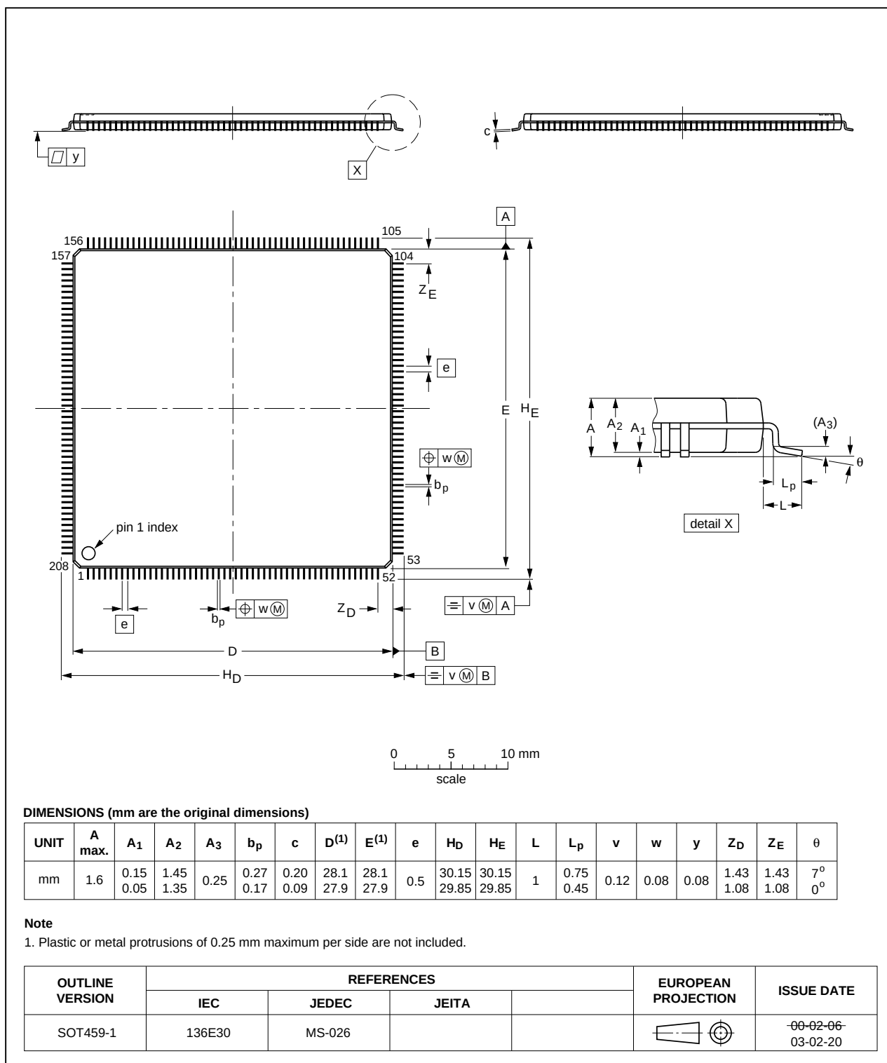
Fig 32. Package outline SOT459-1 (LQFP208)
