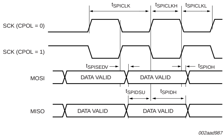
Fig 27. SPI master timing (CPHA = 0)
