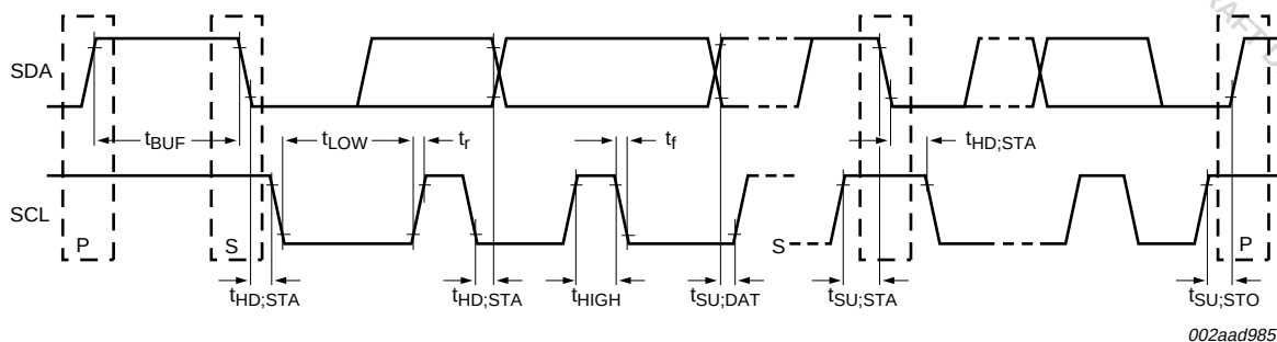
Fig 33. I 2 C-bus pins clock timing
