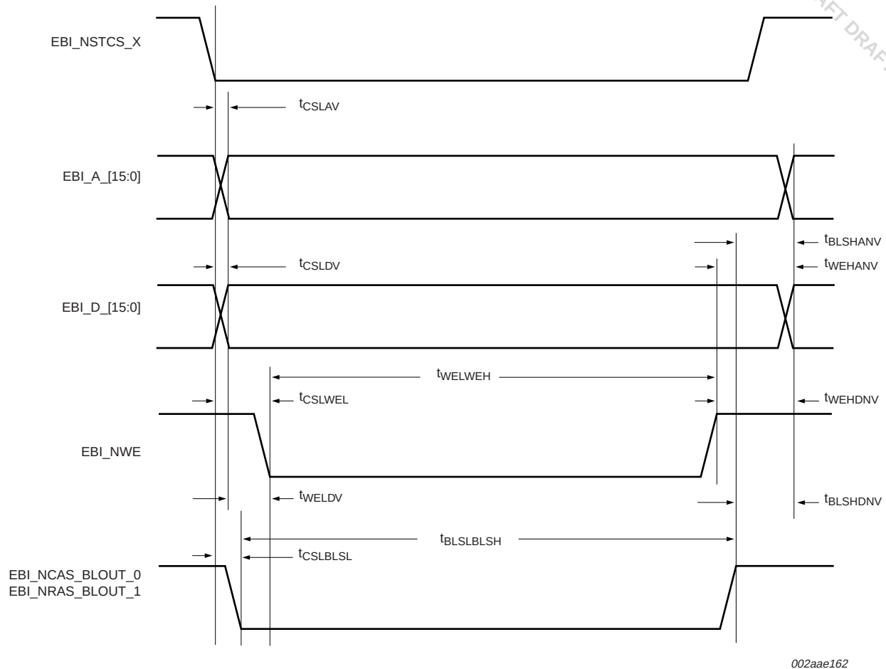
Fig 22. External memory write access to static memory
