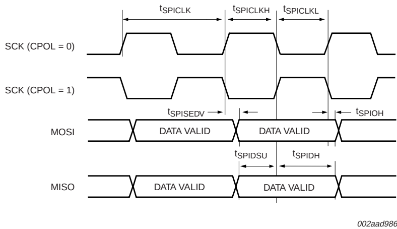
Fig 26. SPI master timing (CPHA = 1)
