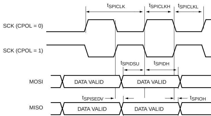
Fig 29. SPI slave timing (CPHA = 0)
