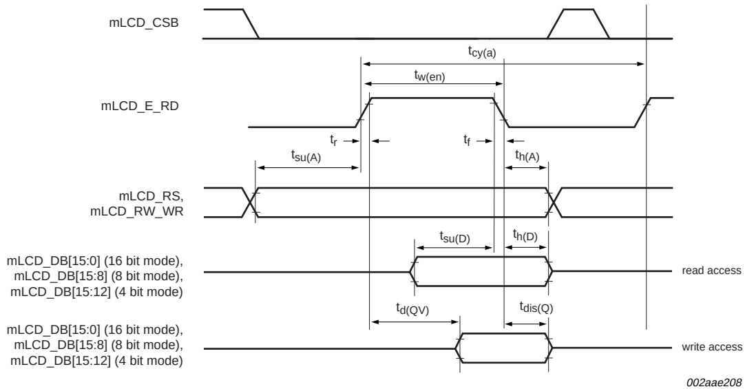
Fig 19. LCD timing (Motorola 6800 mode)
