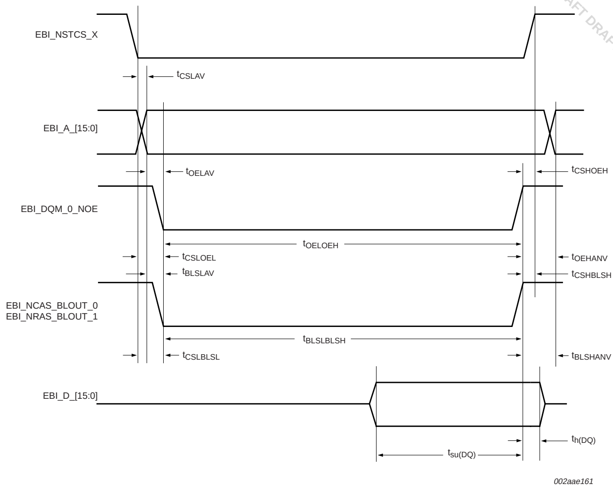
Fig 21. External memory read access to static memory
