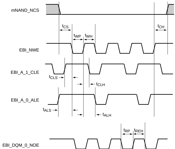
Fig 25. NAND flash controller write and read timing
