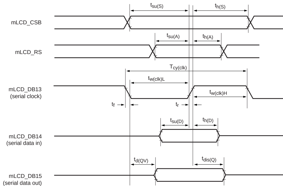
Fig 20. LCD timing (serial mode)
