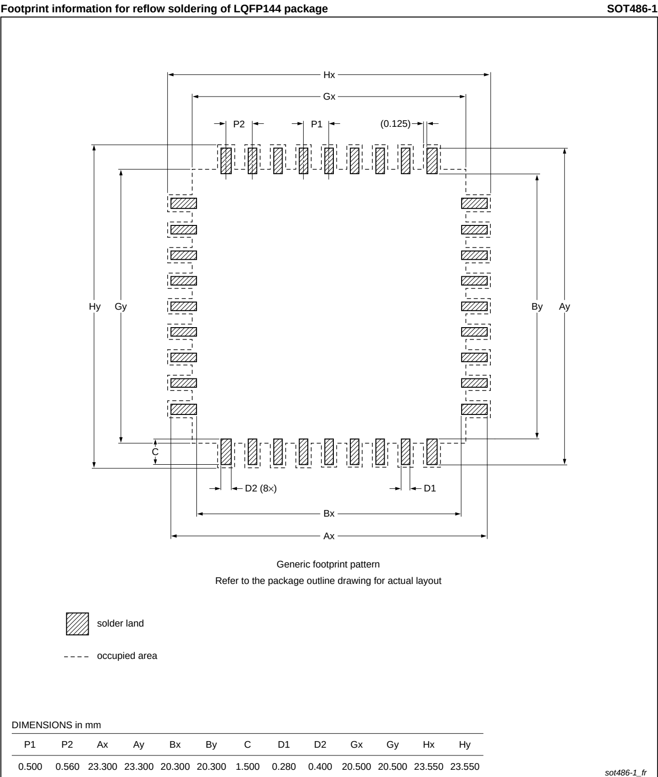
Fig 54. Reflow soldering of the LQFP144 package
