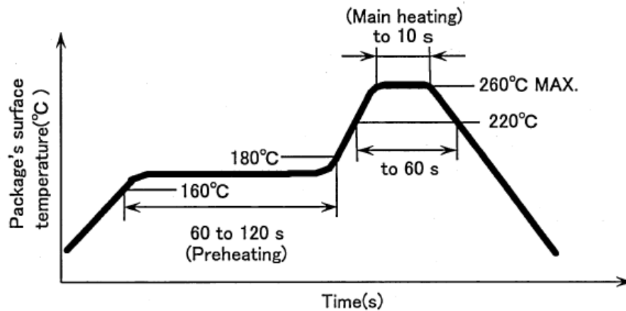
Infrared Reflow Temperature Profile
