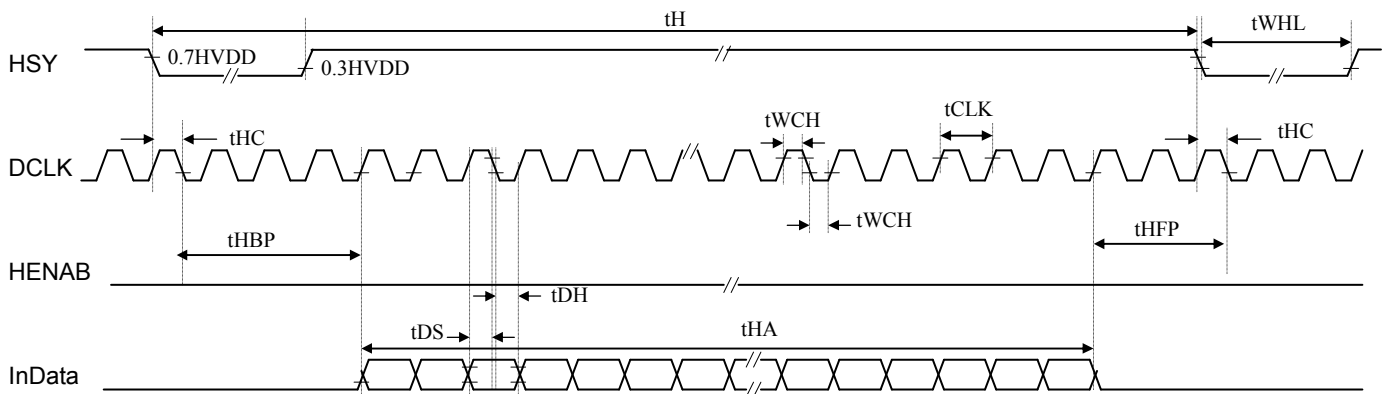
Figure 6-2: WVGA/WQVGA/WEA1/WEA2 Input Data Format (HENAB_Lo fixed/horizontal timing)
