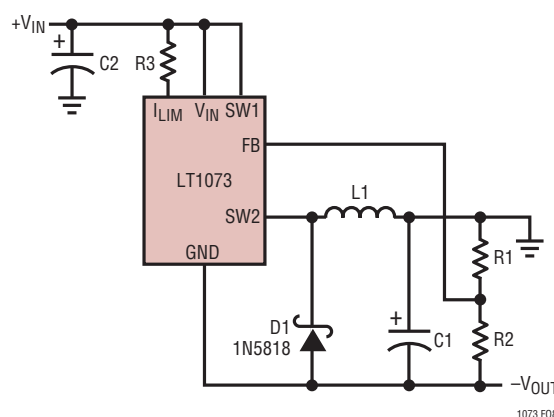
Figure 8. Positive-to-Negative Converter
