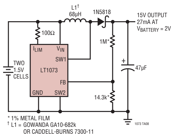
3V to 15V Step-Up Converter
