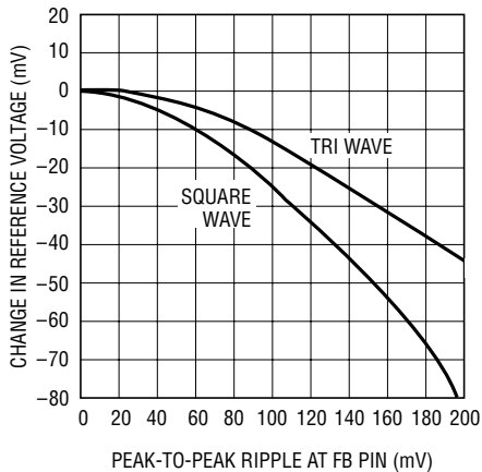
Reference Shift with Ripple Voltage
