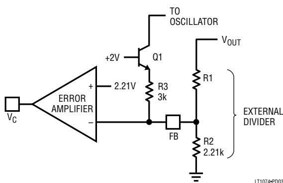
Figure 3. Frequency Shifting
