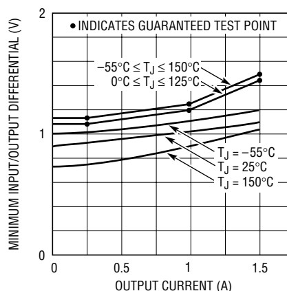
LT1086 Dropout Voltage
