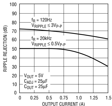
LT1086-5 Ripple Rejection vs Current
