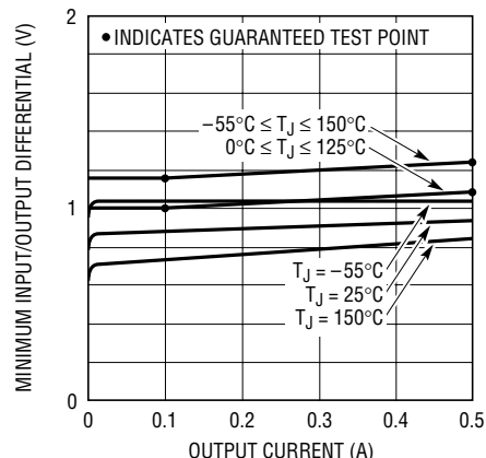
LT1086H Dropout Voltage
