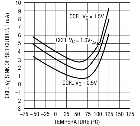
CCFL V_C Offset Sink Current vs Temperature
