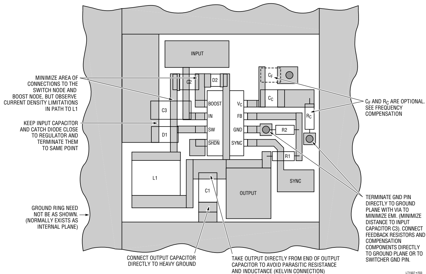
Figure 3. Suggested Layout
