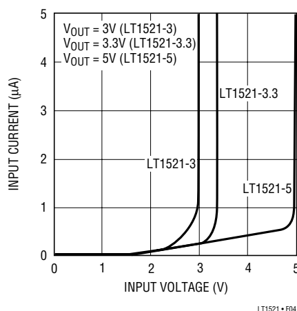
Figure 4. Input Current
