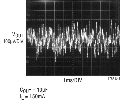
LT1762-5 10Hz to 100kHz Output Noise C_{BYP} = 100 pF
