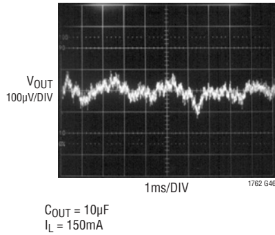
LT1762-5 10Hz to 100kHz Output Noise C_{BYP} = 1000 pF
