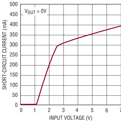
Current Limit
