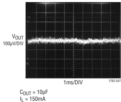
LT1762-5 10Hz to 100kHz Output Noise C_{BYP} = 0.01 \mu F
