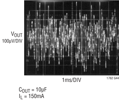
LT1762-5 10Hz to 100kHz Output Noise C_{BYP} = 0
