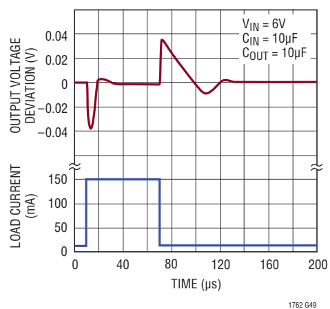
LT1762-5 Transient Response C_{BYP} = 0.01 \mu F
