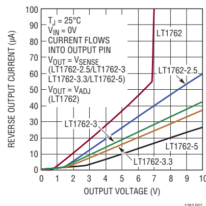
Figure 7. Reverse Output Current
