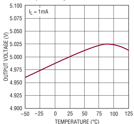
LT1762-5 Output Voltage
