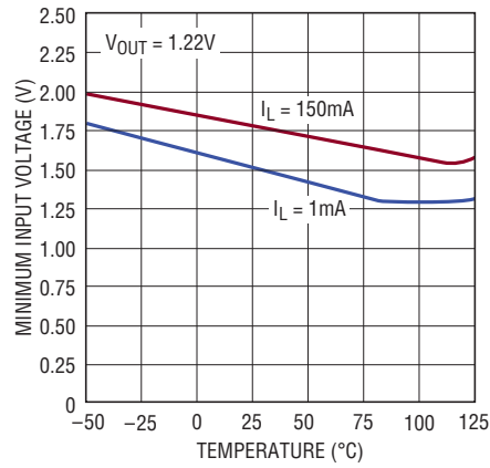
LT1762 Minimum Input Voltage
