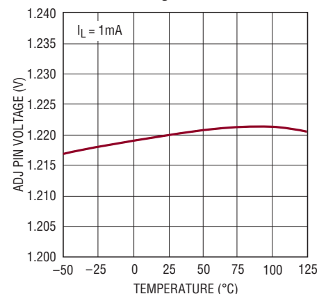
LT1762 ADJ Pin Voltage
