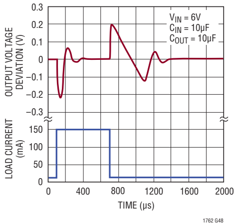
LT1762-5 Transient Response C_{BYP} = 0
