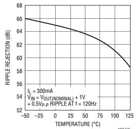
Ripple Rejection
