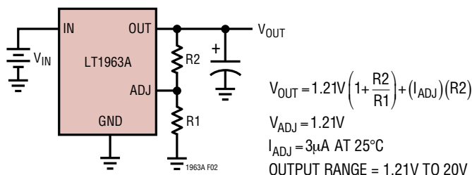
Figure 2. Adjustable Operation
