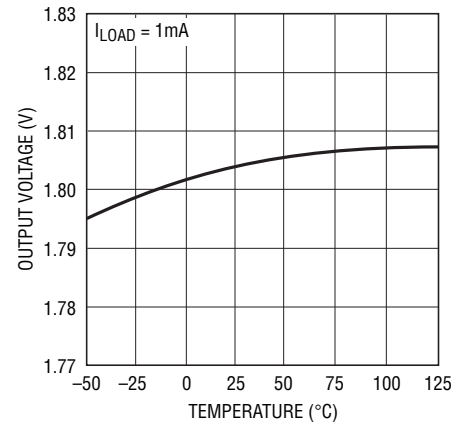
Output Voltage
