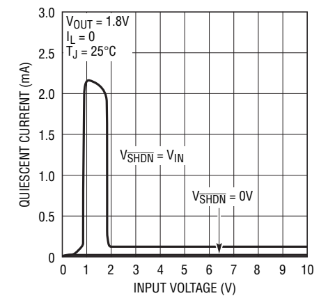
Quiescent Current
