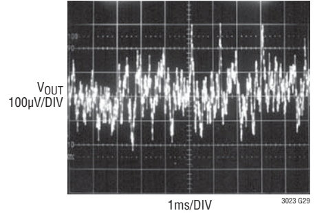
10Hz to 100kHz Output Noise C BYP = 100pF
