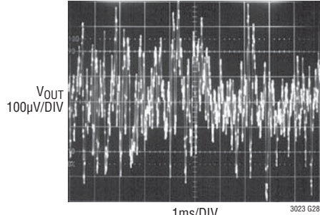
10Hz to 100kHz Output Noise C BYP = 0
