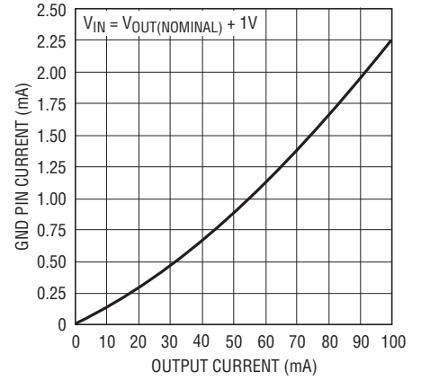
Output 2 GND Pin Current vs I_{LOAD}
