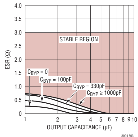
Figure 3. Output 1 Stability
