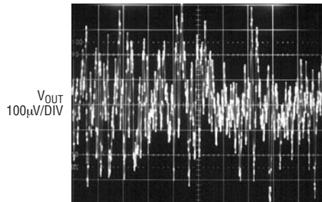
C_{OUT} = 10µF 1ms/DIV 3028 G42 I_L = FULL LOAD V_{OUT} SET FOR 5V
