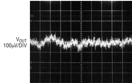
C_{OUT} = 10µF 1ms/DIV 3028 G44 I_L = FULL LOAD V_{OUT} SET FOR 5V
