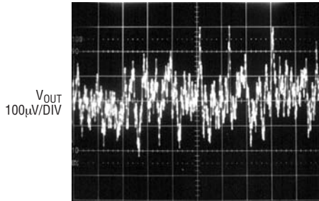
C_{OUT} = 10µF 1ms/DIV 3028 G43 I_L = FULL LOAD V_{OUT} SET FOR 5V
