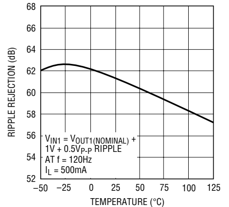
Output 1 Ripple Rejection
