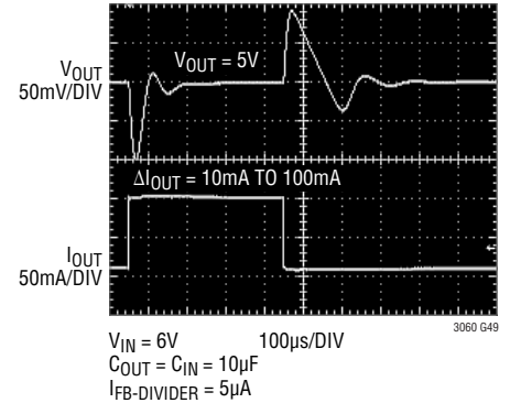
LT3060-5 Transient Response, C_{FF} = 0
