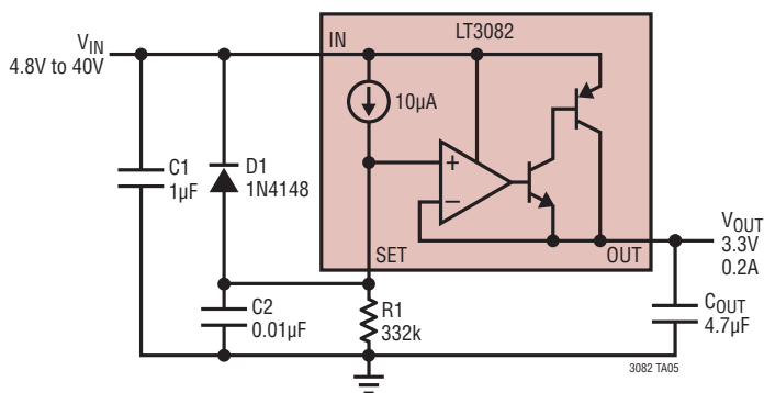
Adding Soft-Start
