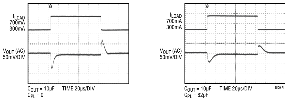
Figure 11. Transient Load Response with Different Combinations of C_{OUT} and C_{PL} Load Current Step from 300mA to 700mA R1 = 10\text{k} , R2 = 32.4\text{k} , V_{IN} = 12\text{V} , V_{OUT} = 3.3\text{V} , f_{SW} = 2.0\text{MHz}
