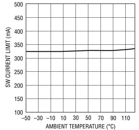
SW3 Current Limit
