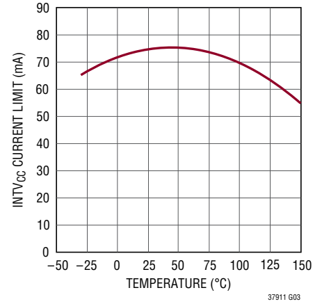
INTV CC Current Limit vs Temperature
