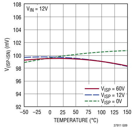
V (ISP-ISN) Threshold vs Temperature
