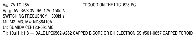
Figure 12. LTC1628 High Efficiency Low Noise 5V/3A, 3.3V/5A, 12/120mA Regulator
