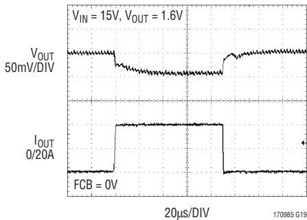
Load Step
