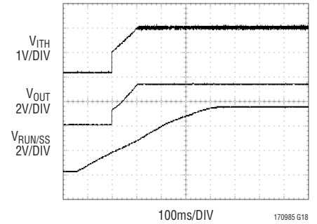
Soft-Start Up
