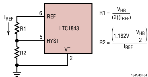
Figure 4. Programmable Hysteresis
